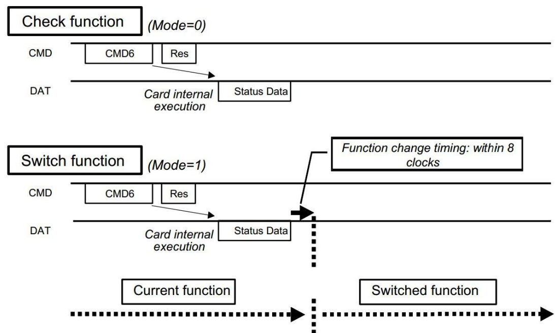
Figure 4-4: Use of Switch Command
